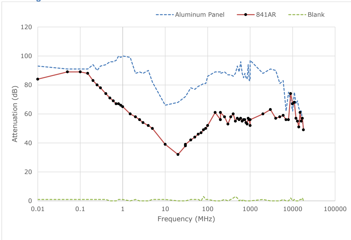
Figure 2. Attenuation of 841AR coating at different frequencies
